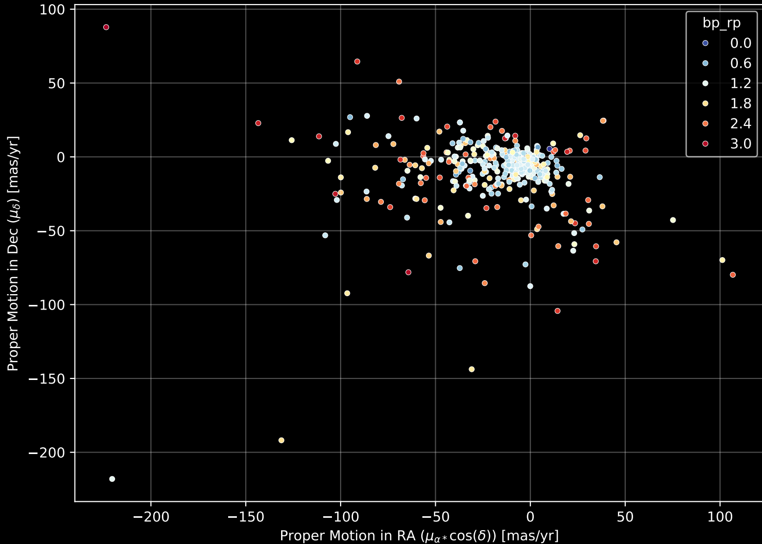
APOGEE DR17 Field: [240+75] Proper Motion Diagram (n= 402)
