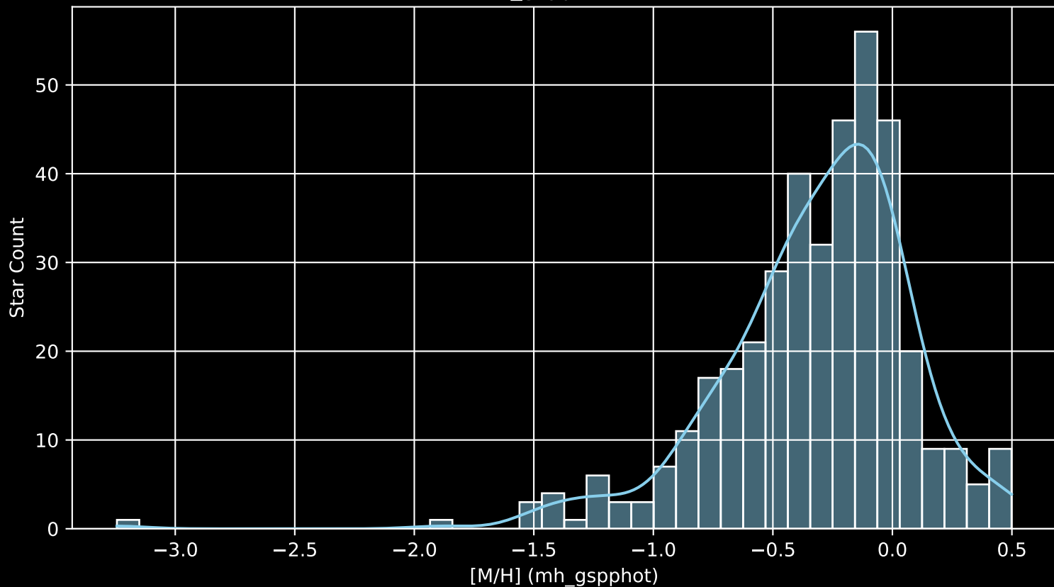
APOGEE DR17 Field: [240+75 [M/H] (mh_gspphot) (n= 397)
