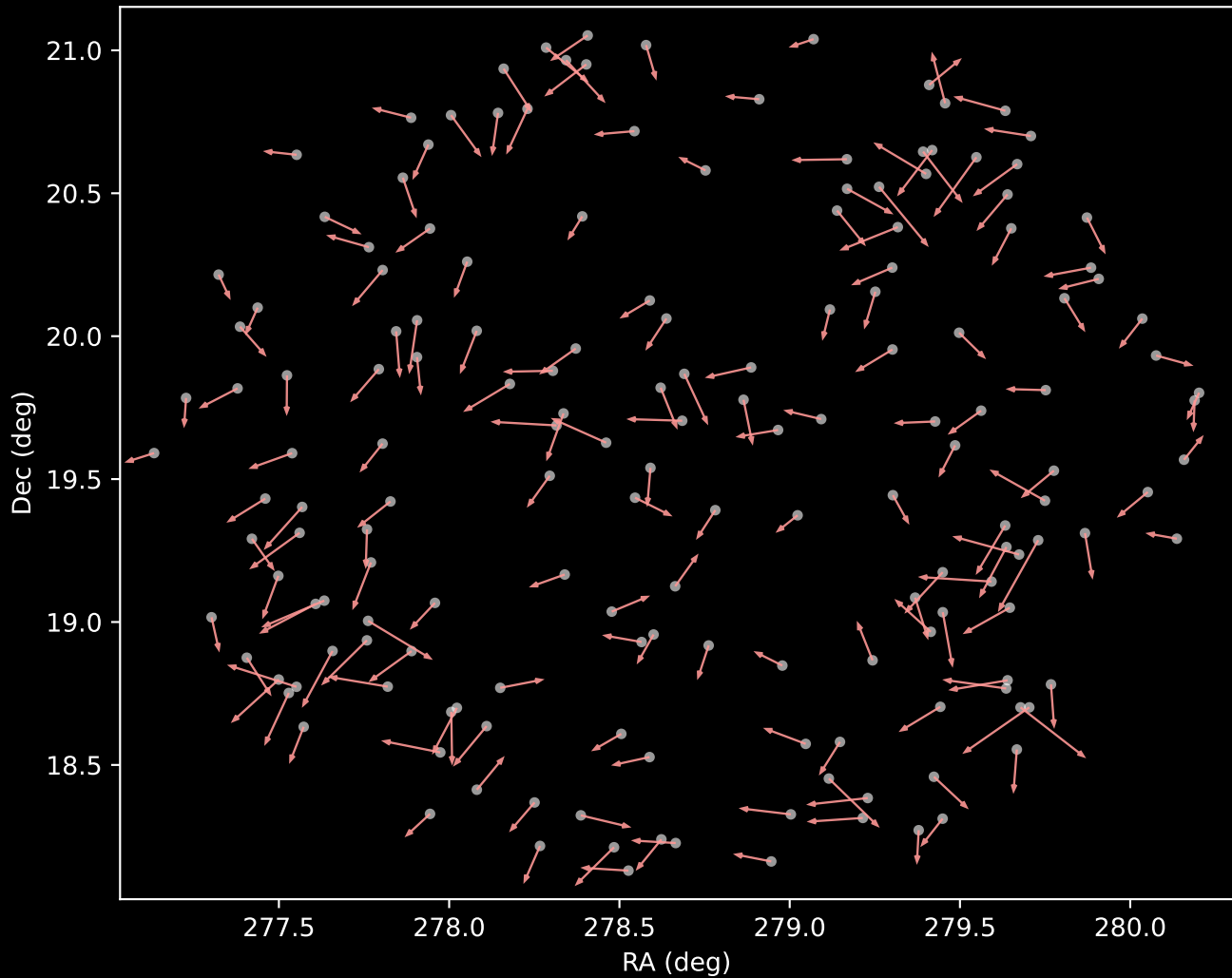
APOGEE DR17 Cluster 7 Proper Motion Vectors (n=170)
