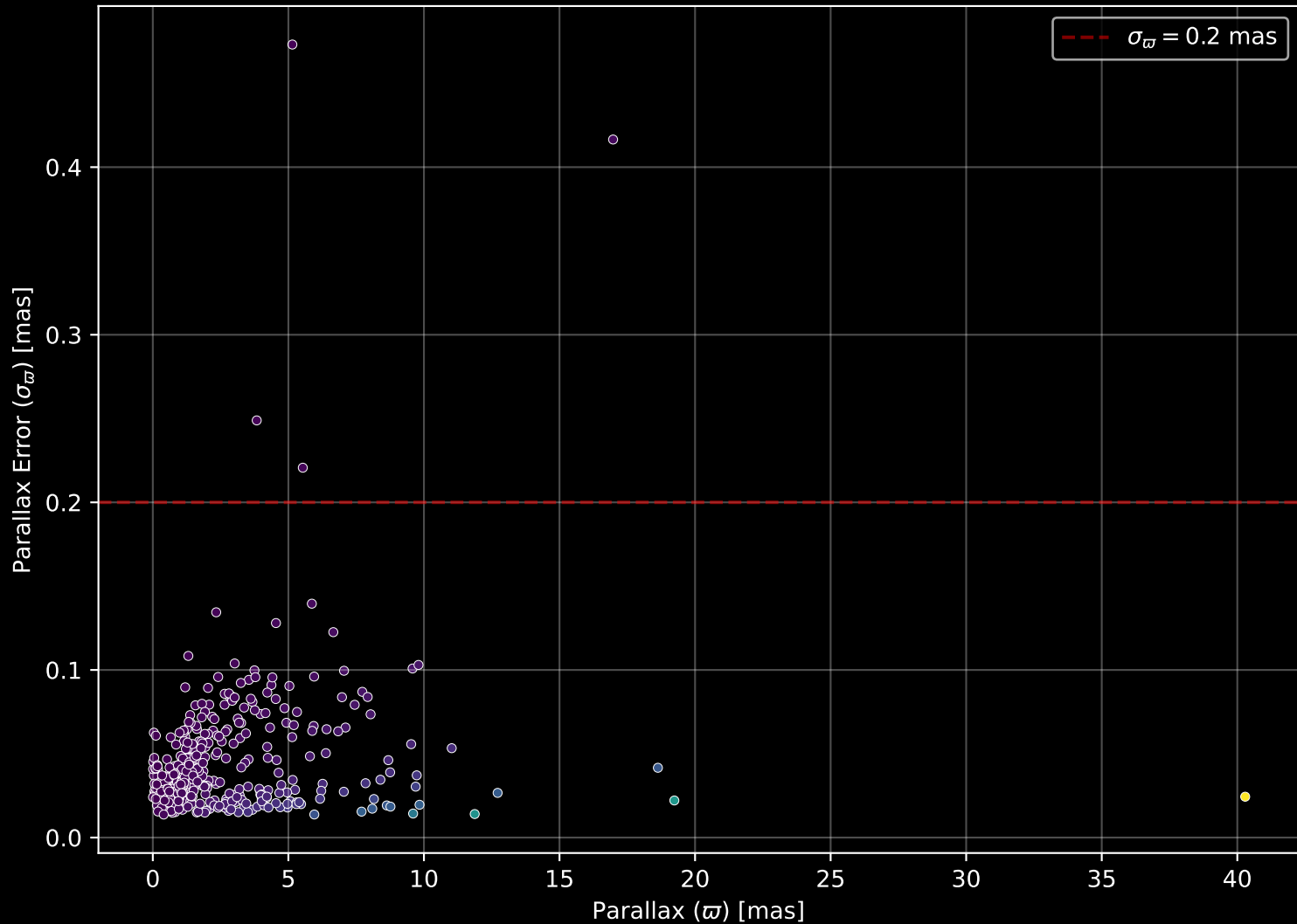
APOGEE DR17 Field: [240+75] Parallax Quality (n= 402)
