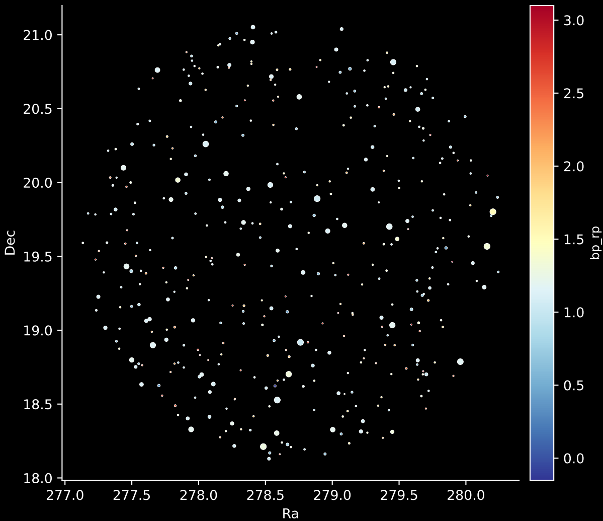
APOGEE DR17 Field: [240+75] Stars: 402
