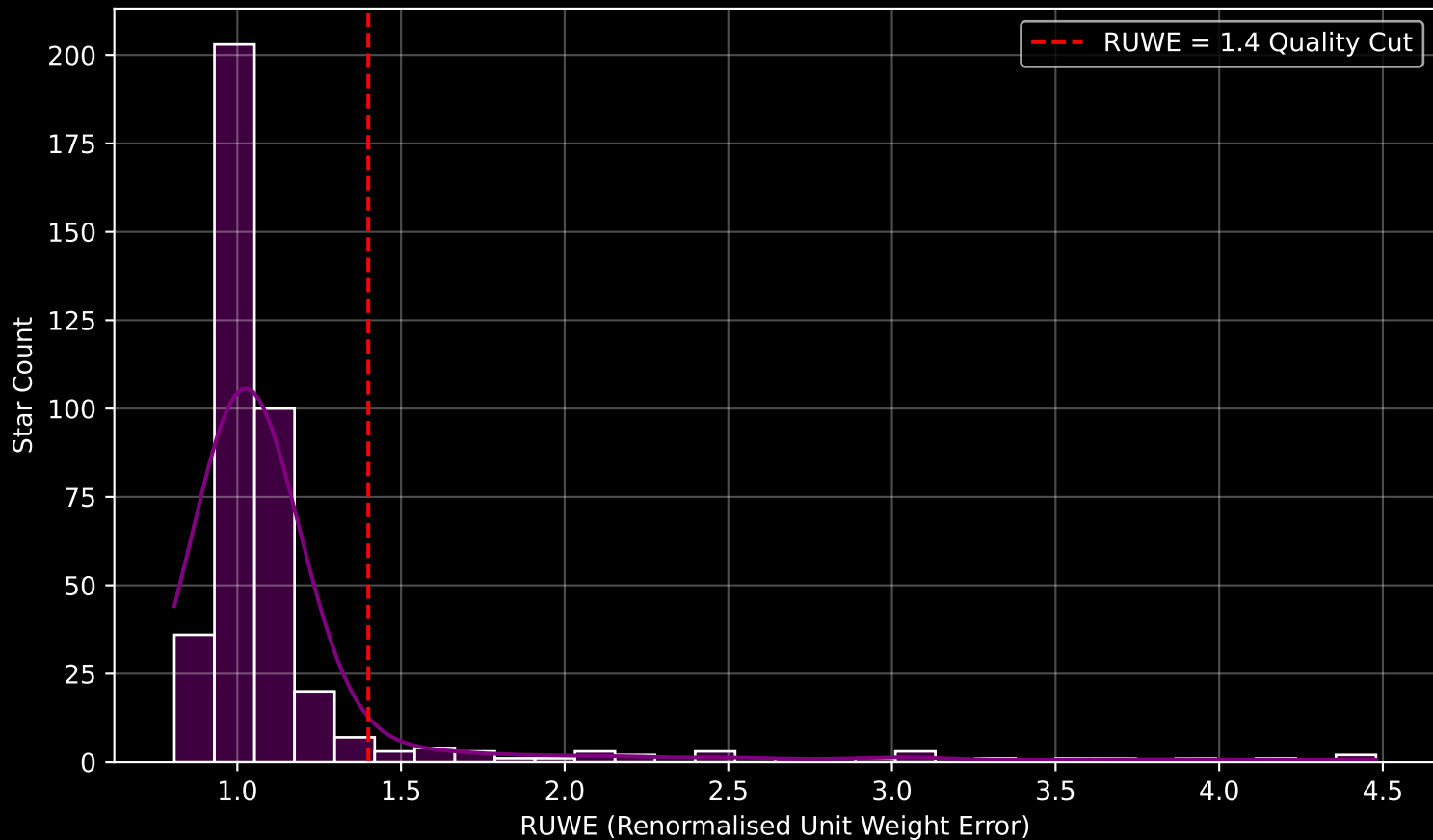
GAPOGEE DR17 Field [240+75] RUWE Distribution (n= 398)
