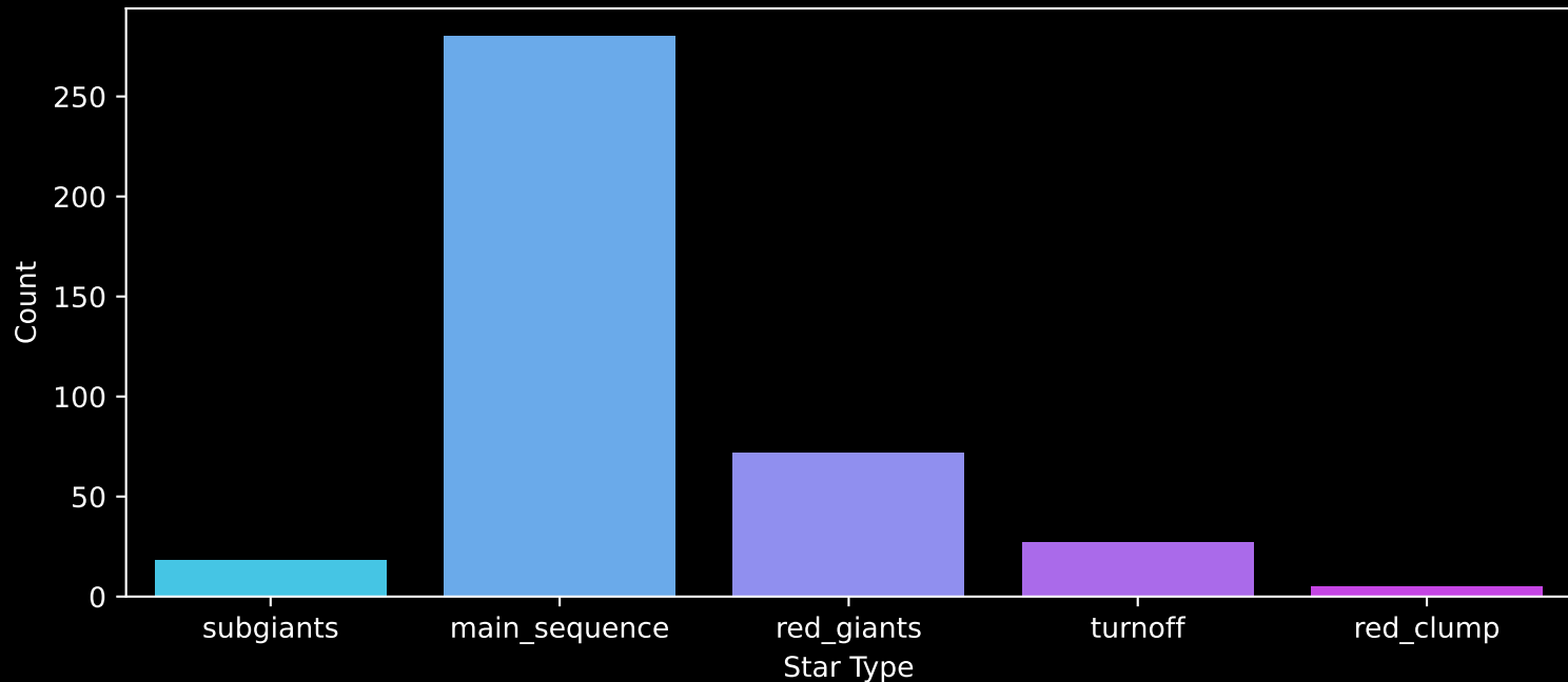
APOGEE DR17 Field: [240+75] Count plot of Star Type
